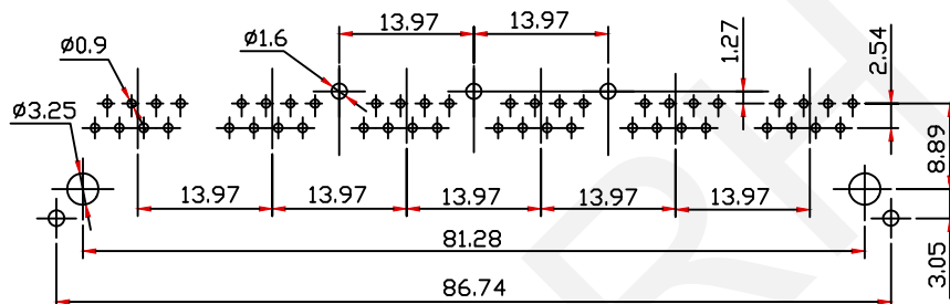
PCB Layout
