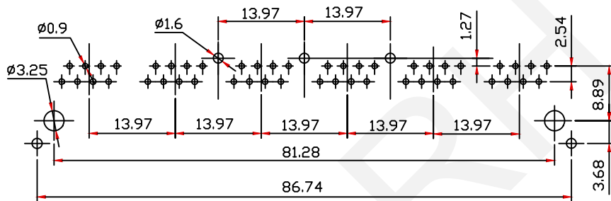
PCB Layout
