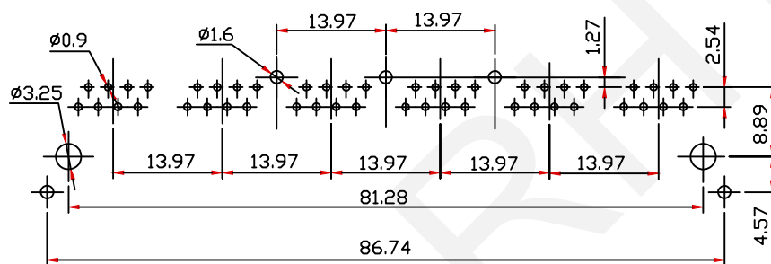
PCB Layout
